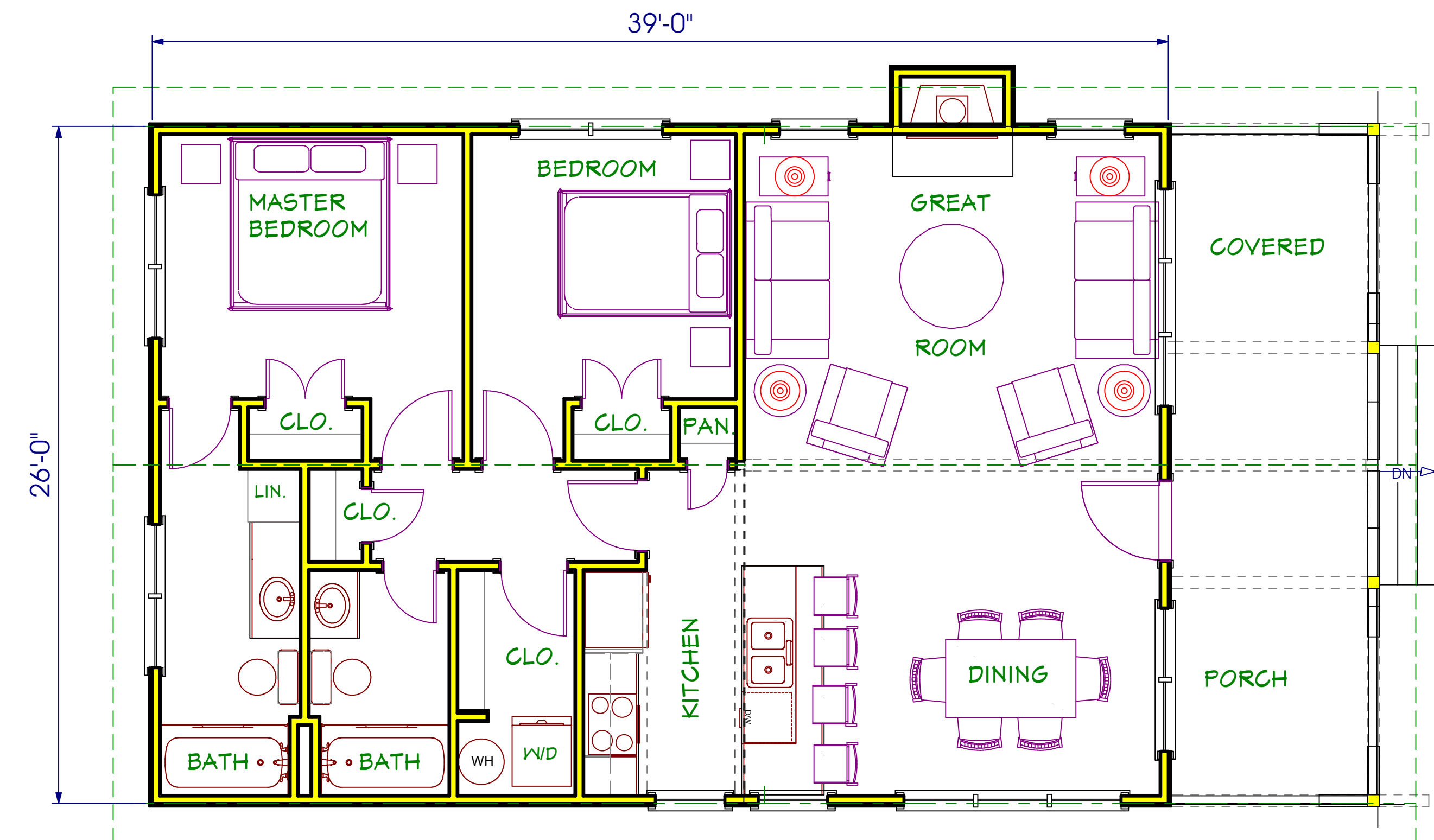
FIRST FLOOR PLAN 1,014 SQ.FT.
