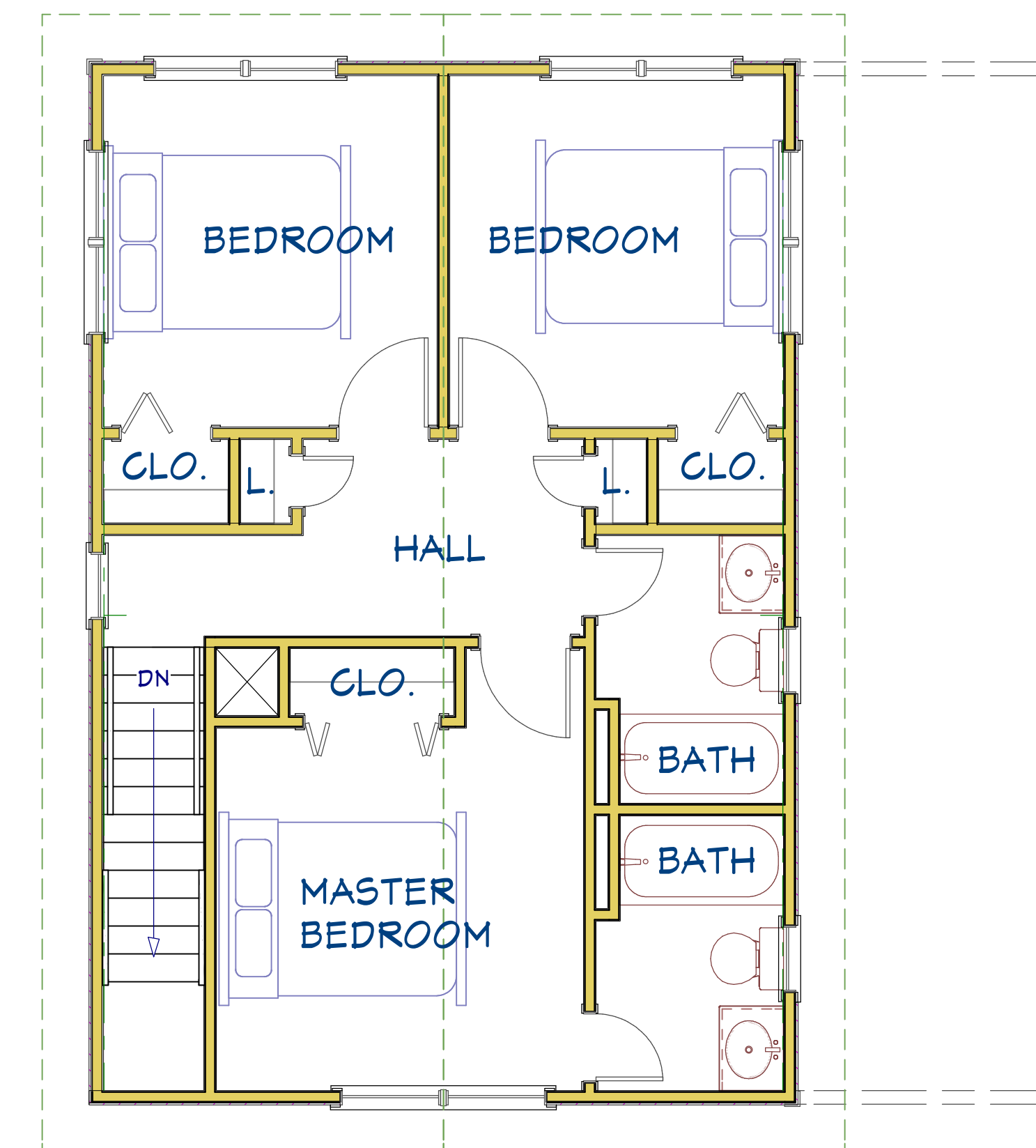
SECOND FLOOR PLAN 606 SQUARE FEET
