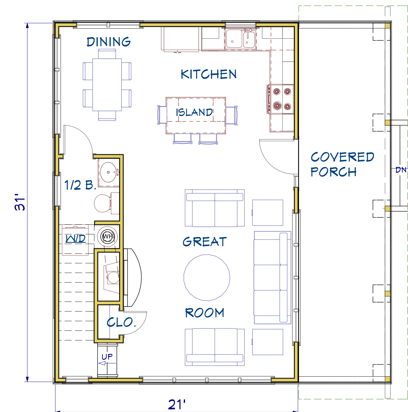
FIRST FLOOR PLAN 651 SQUARE FEET
