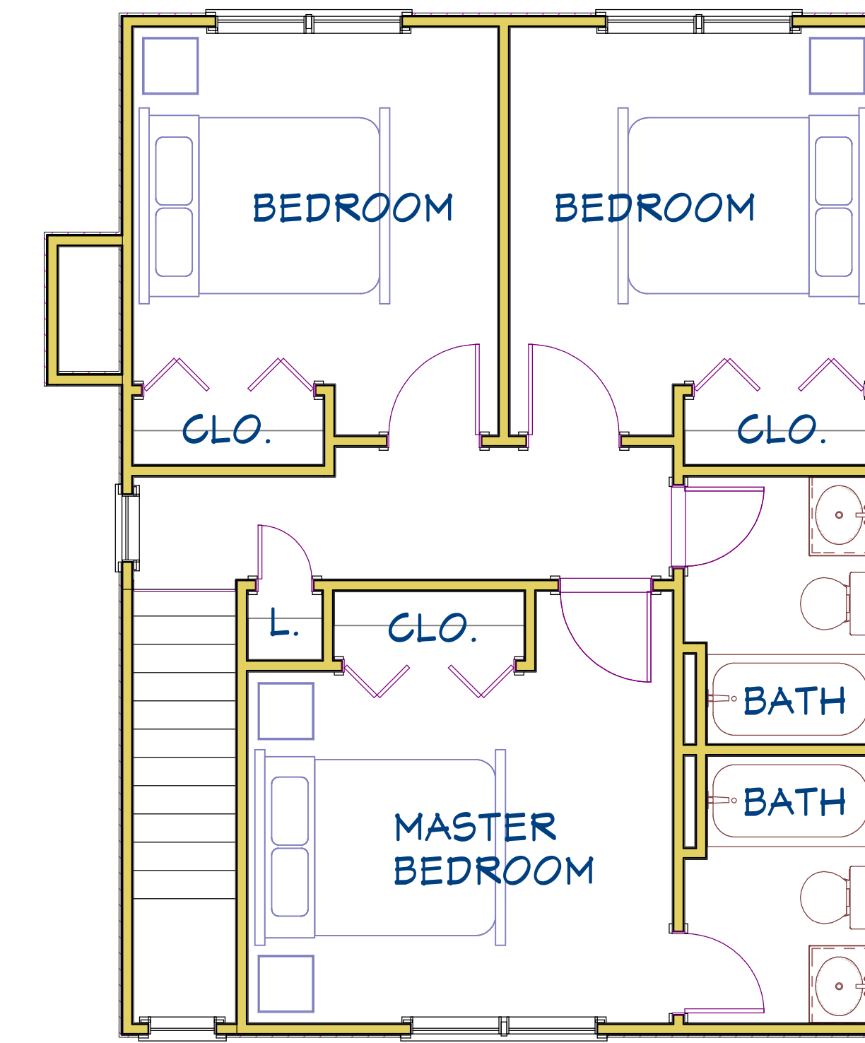
SECOND FLOOR PLAN 630 SQUARE FEET
