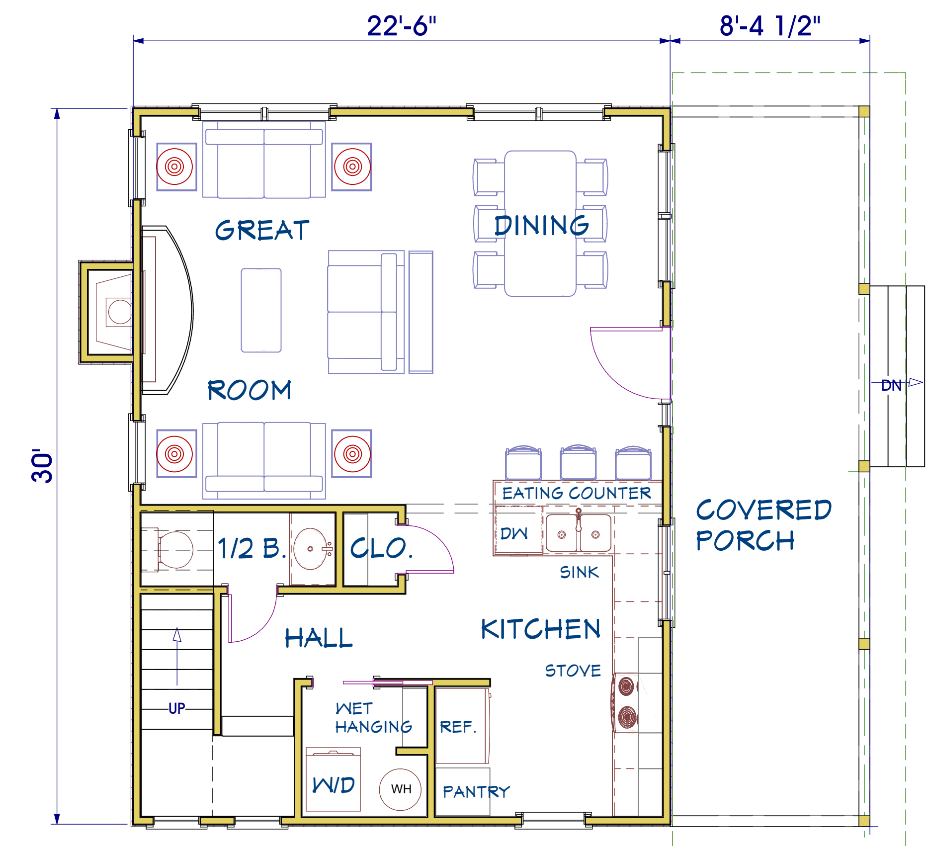
FIRST FLOOR PLAN 675 SQUARE FEET
