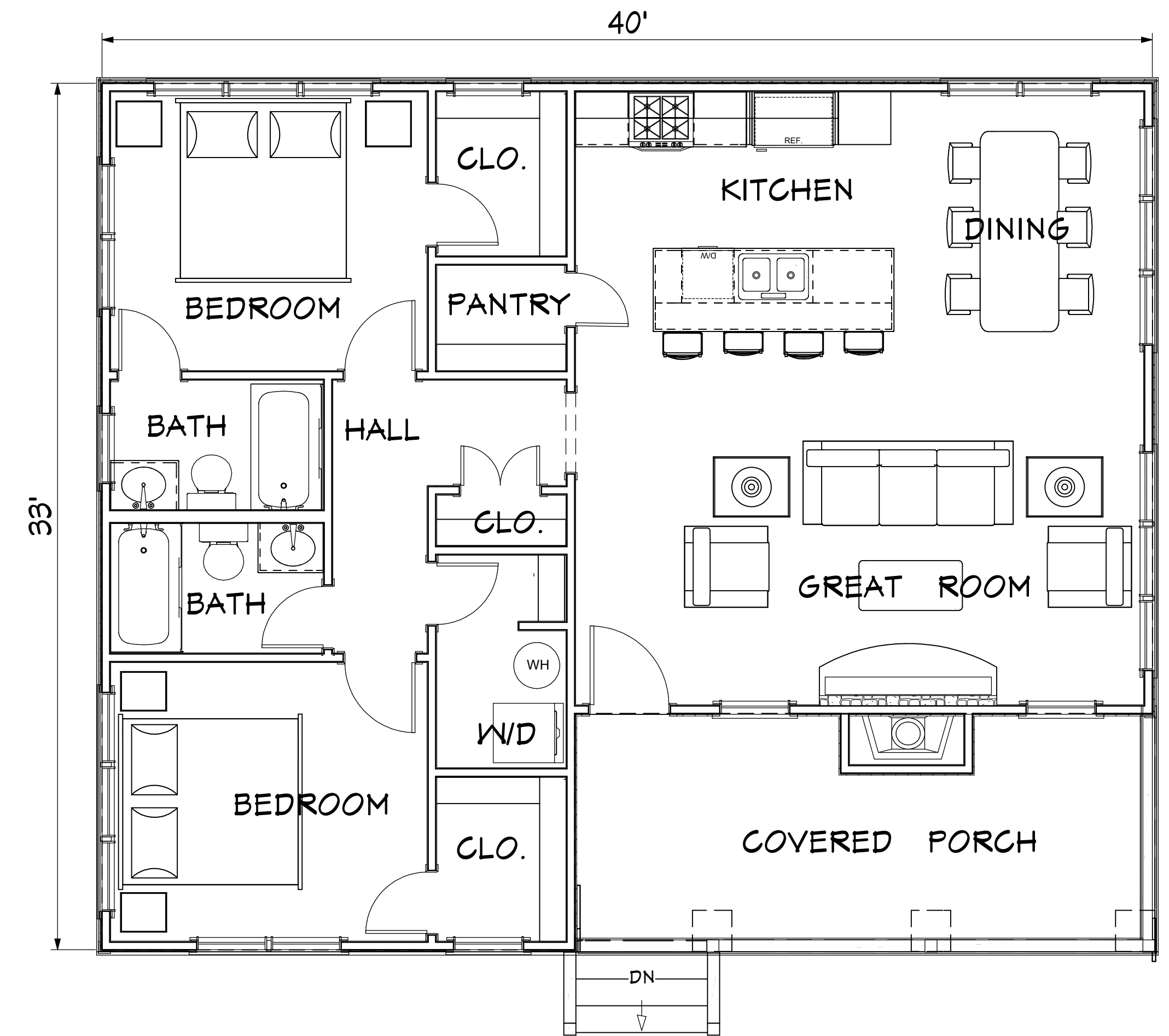
FLOOR PLAN 1,123 SQUARE FEET
