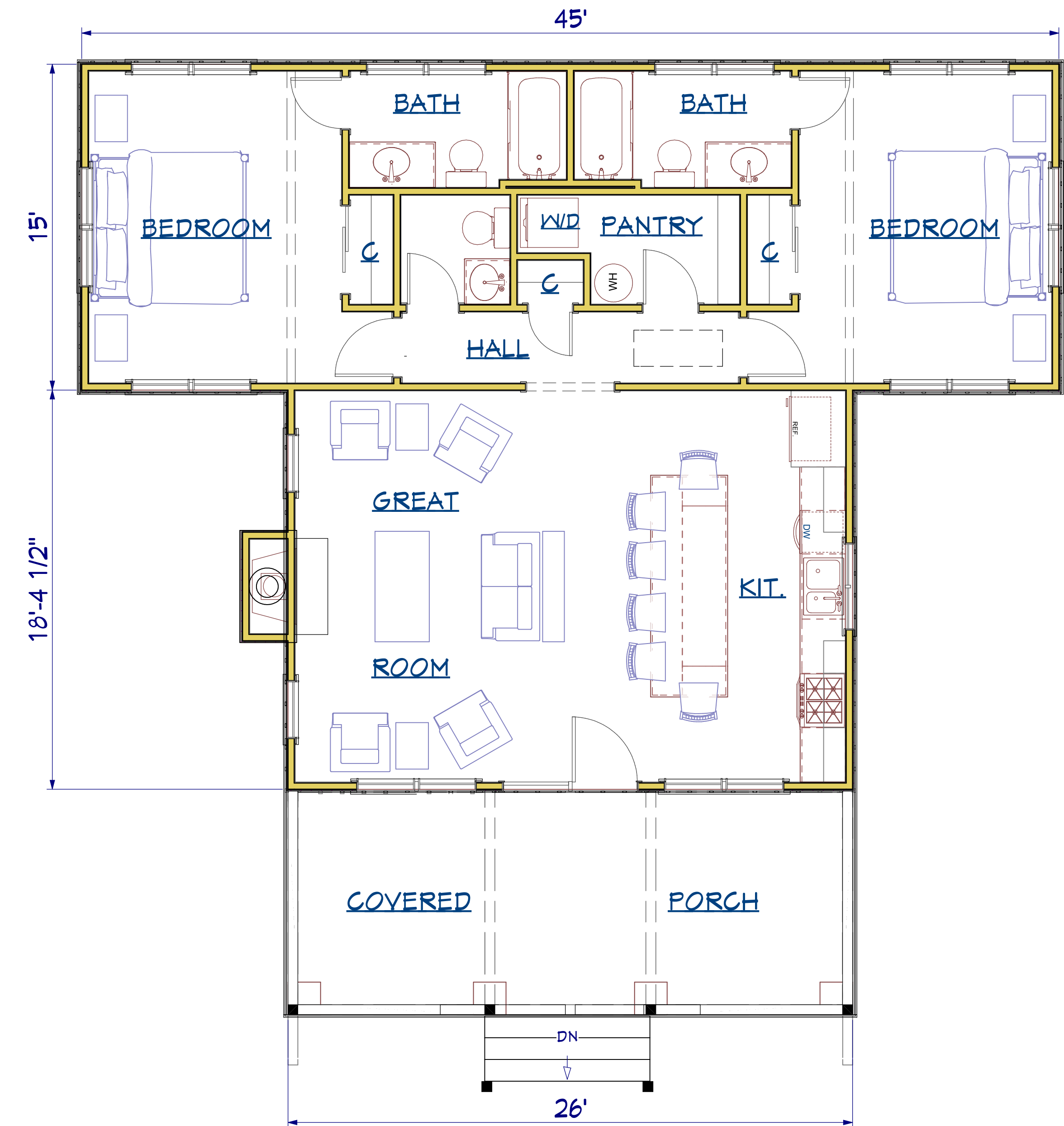
FLOOR PLAN 1,152 SQUARE FEET
