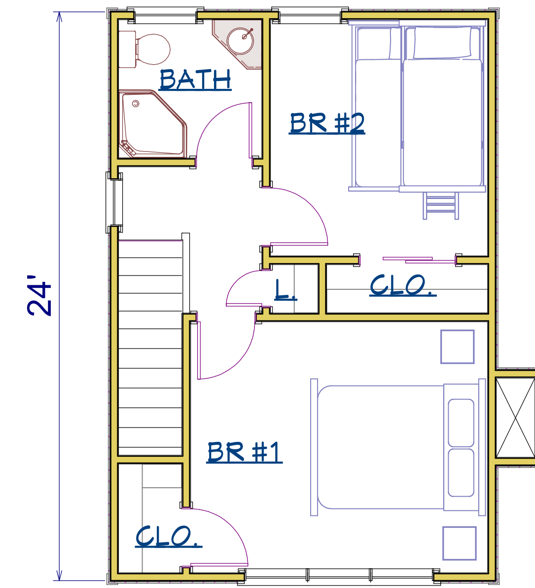
SECOND FLOOR PLAN 390 SQUARE FEET
