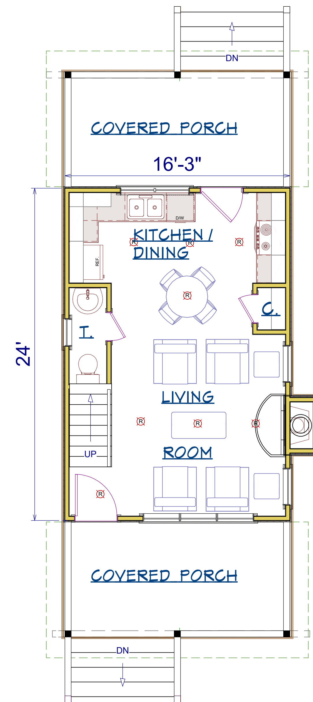
FIRST FLOOR PLAN 390 SQUARE FEET
