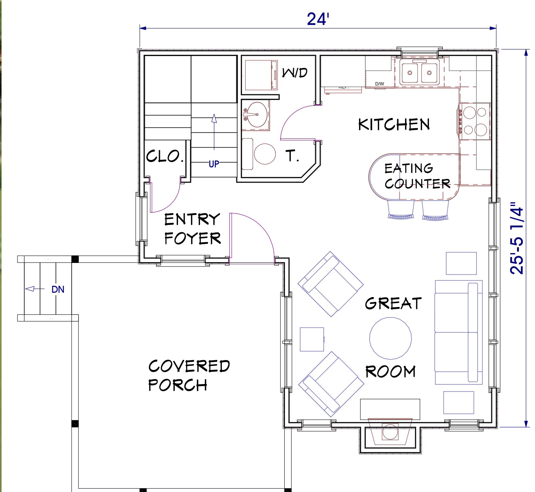
FIRST FLOOR PLAN 507 SQUARE FEET
