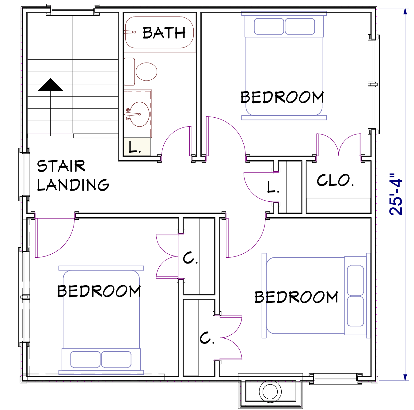
SECOND FLOOR PLAN 608 SQUARE FEET
