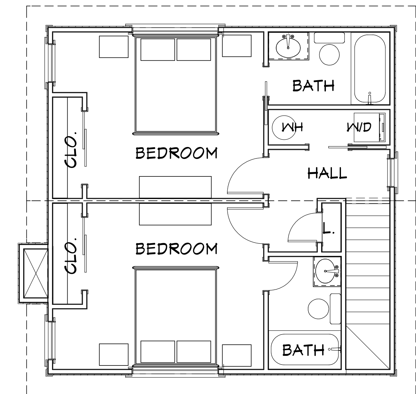
SECOND FLOOR PLAN 536 SQUARE FEET
