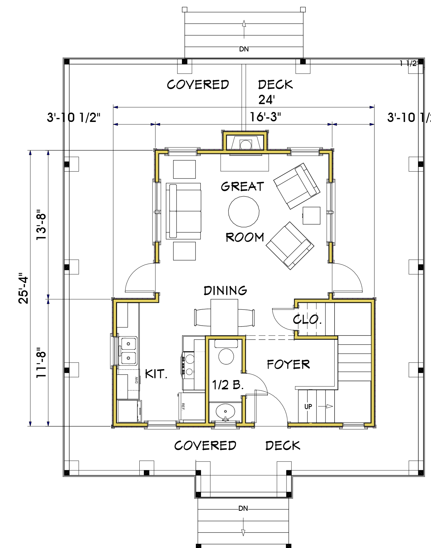
FIRST FLOOR PLAN 502 SQUARE FEET
