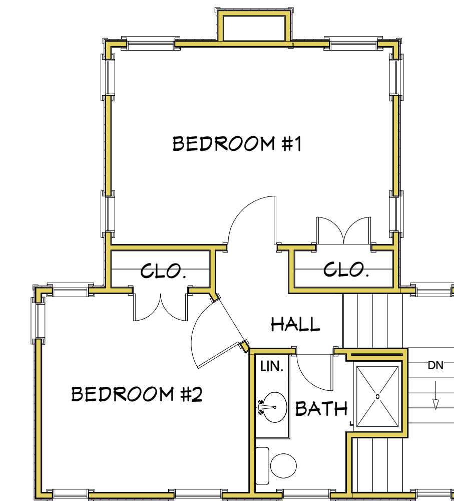
SECOND FLOOR PLAN 443 SQUARE FEET
