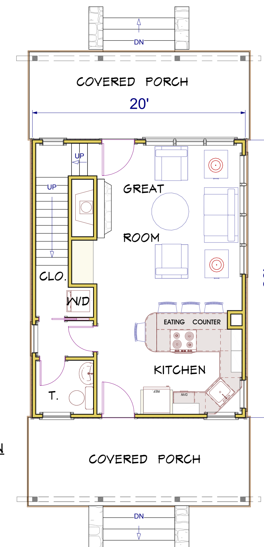
FIRST FLOOR PLAN 520 SQUARE FEET
