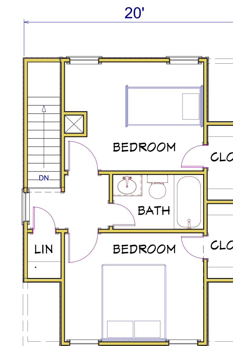
SECOND FLOOR PLAN 431 SQUARE FEET
