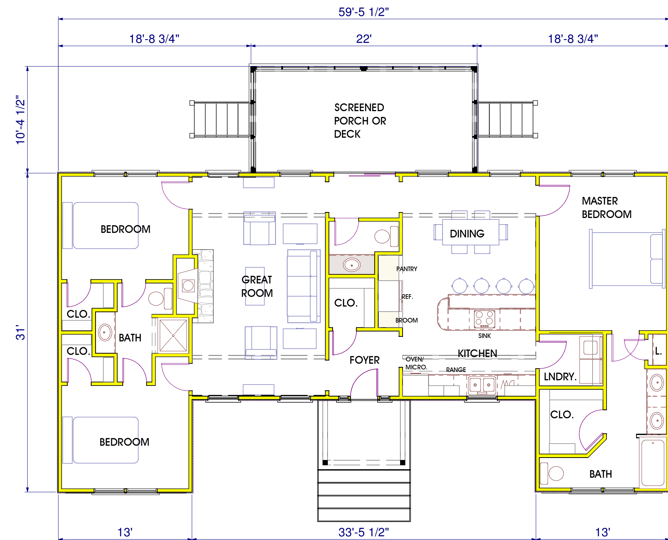
FLOOR PLAN 1242 SQUARE FEET
