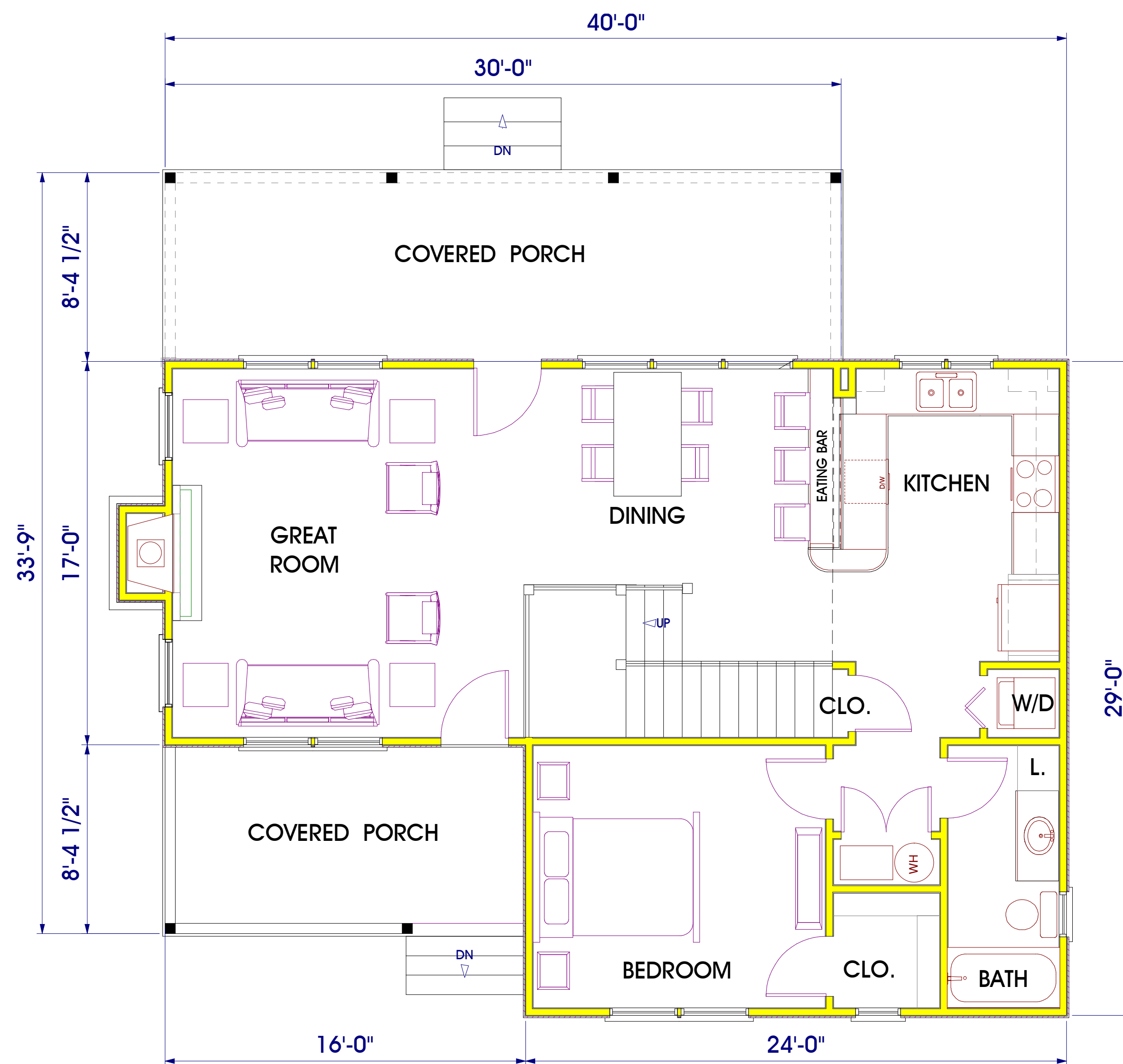
FIRST FLOOR PLAN 696 SQUARE FEET
